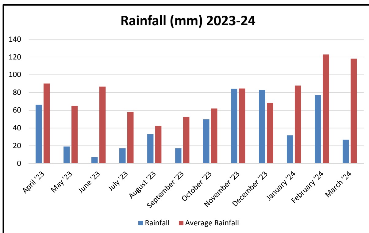
Figure 2: Rainfall YEM 2024
