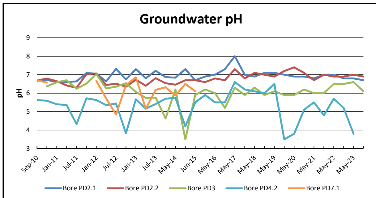
Figure 11: Groundwater pH
