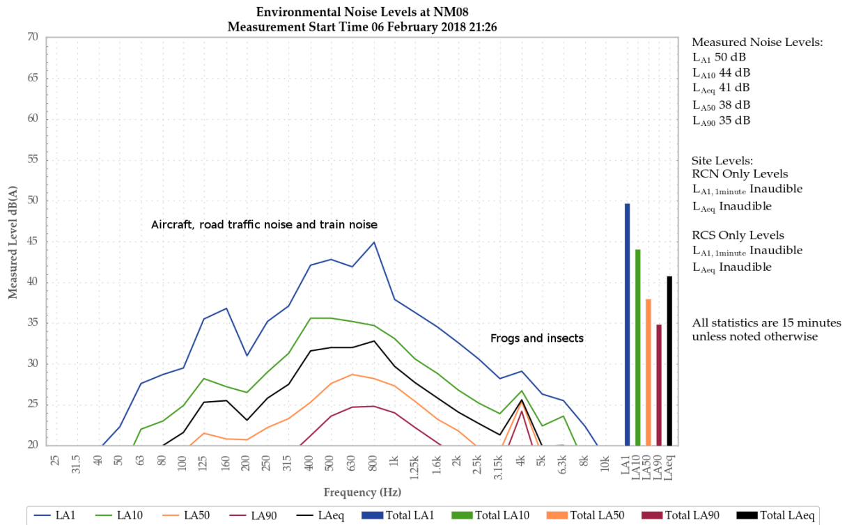
Figure 7: Environmental Noise Levels, NM08 – Cnr Belmadar Way and Maison Dieu Road, Maison Dieu
