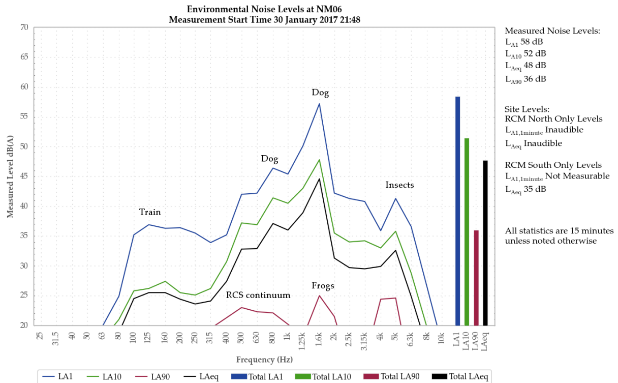
Figure 4: Environmental Noise Levels, NM06 – 427 Bridgman Road, Obanvale
