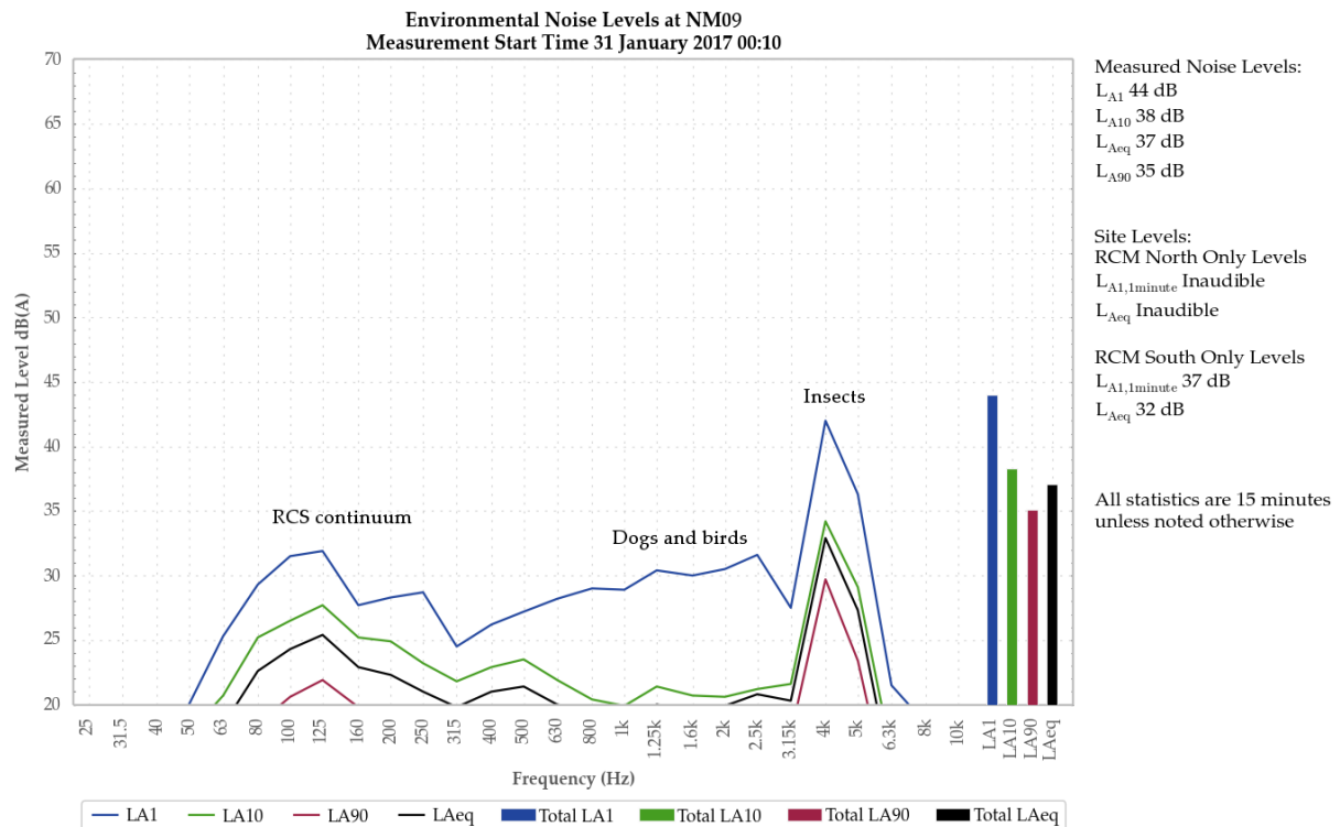
Figure 7: Environmental Noise Levels, NM09 – Llanrian Drive, Gowrie
