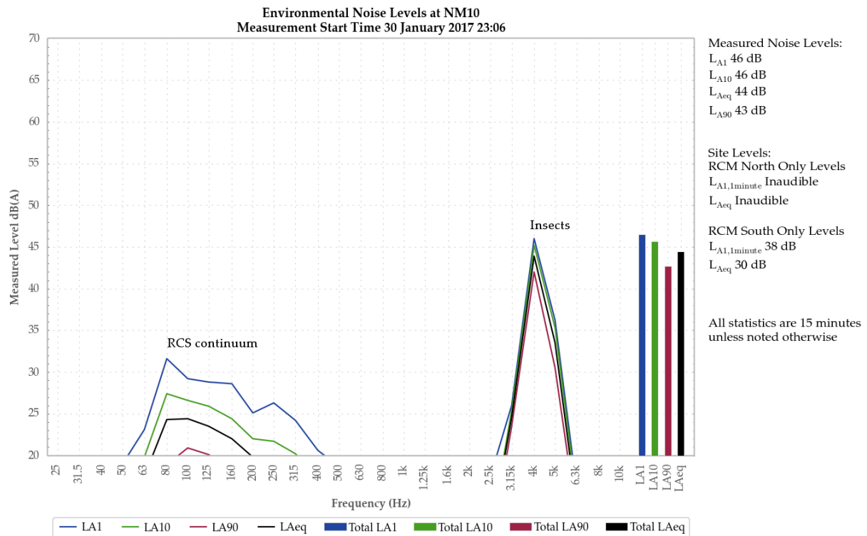
Figure 8: Environmental Noise Levels, NM10 – End of Dights Crossing Road, Maison Dieu
